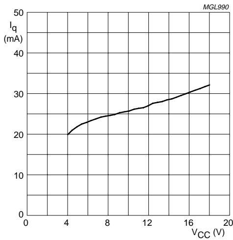
Fig 3. Quiescent supply current as function of supply voltage.
