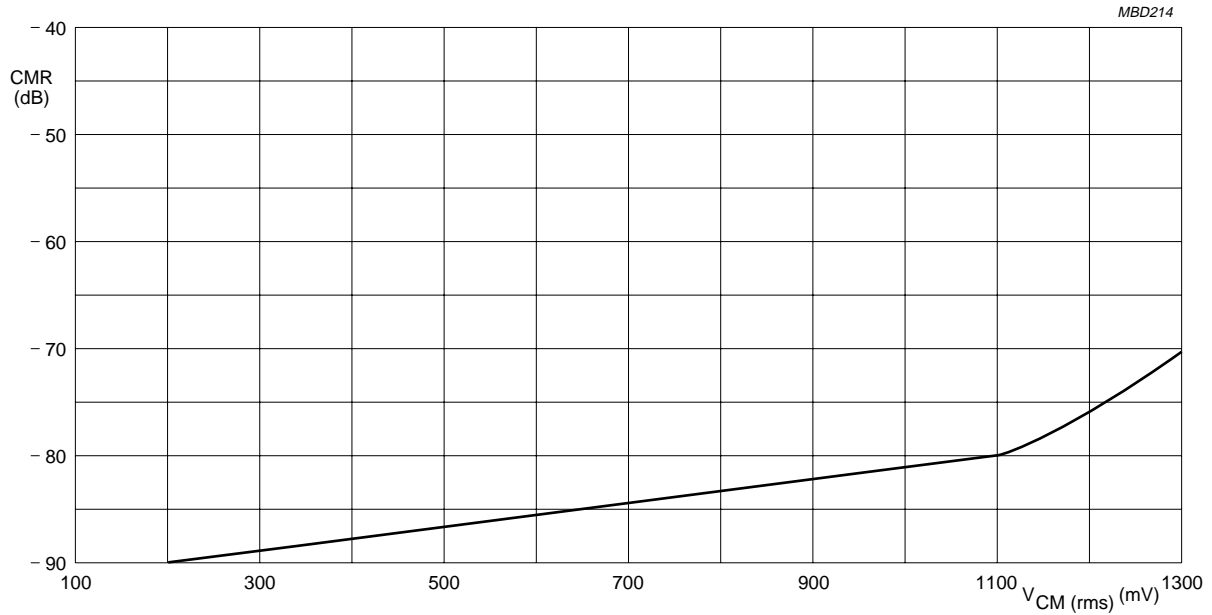
Fig.7 Common-mode rejection as a function of common-mode input voltage; f = 1 kHz; R_s = 0 \Omega .
