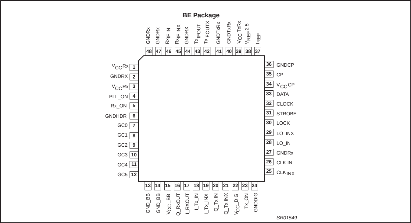
Figure 1. Pin Configuration
