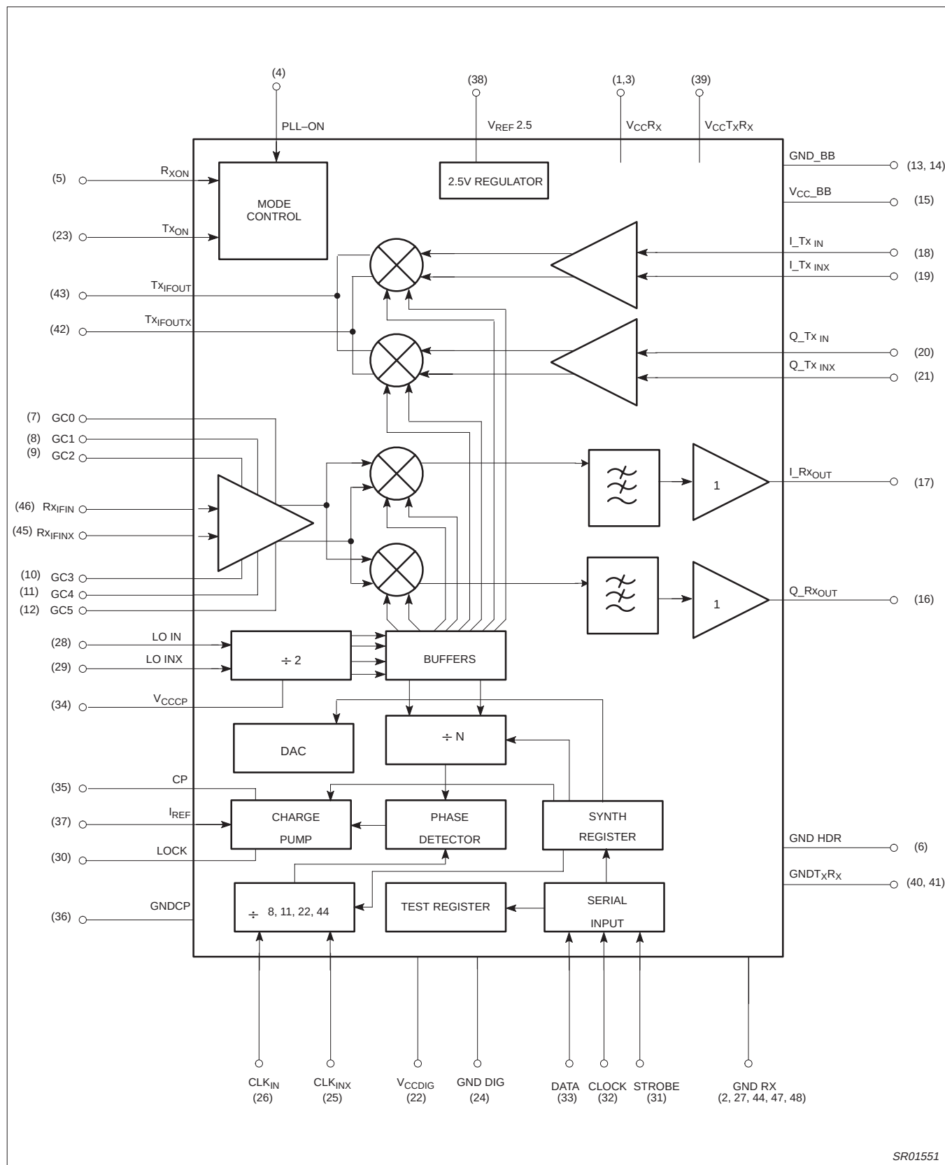
Figure 2. Block Diagram
