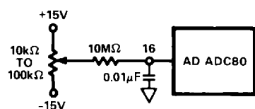
Figure 9. Gain Adjustment Circuit
