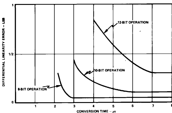
Figure 2b. Change in Differential Linearity vs. Conversion Speed (AD5240)
