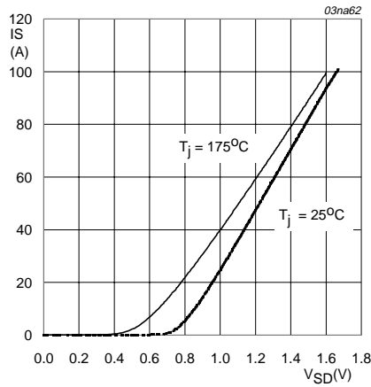
Fig 15. Reverse diode current; typical values.
