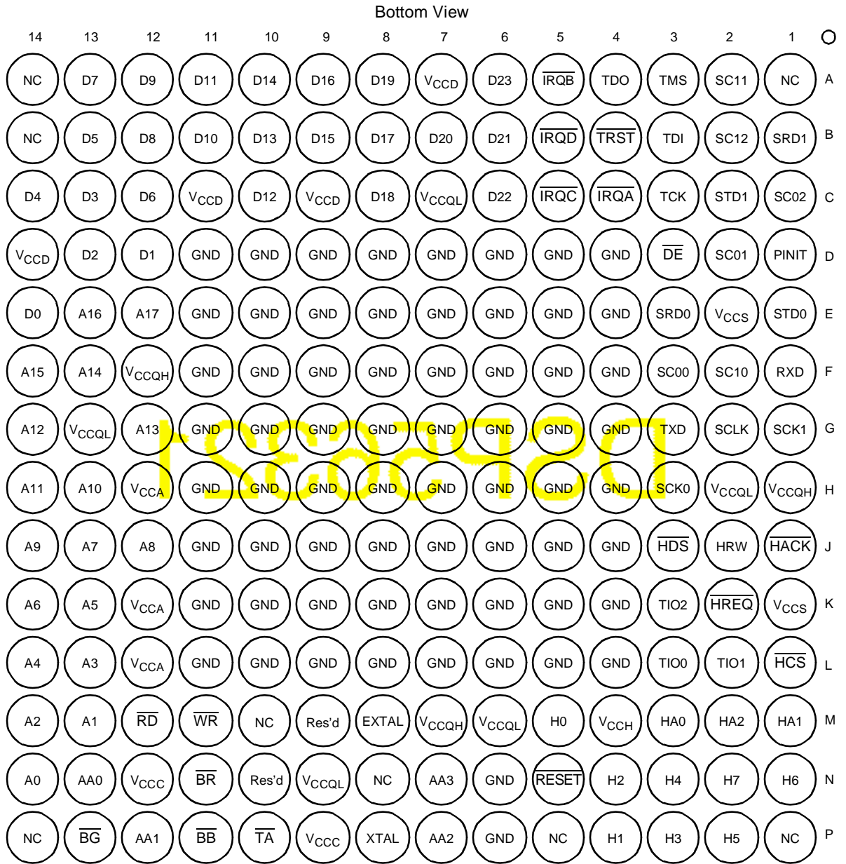
Figure 3-2. DSP56321 FC-PBGA Package, Bottom View
