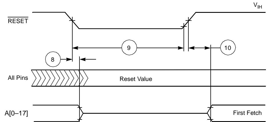
Figure 2-3. Reset Timing
