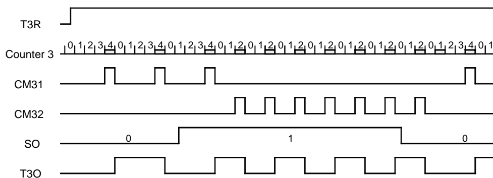
Figure 58. FSK Modulation
