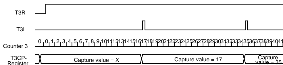
Figure 62. External Capture Mode
