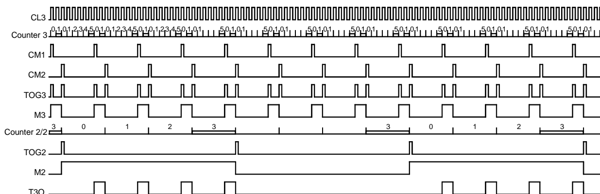
Figure 89. Burst Modulation 1
