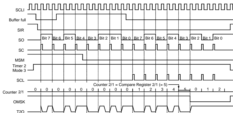
Figure 80. Biphase Modulation
