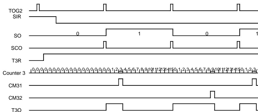
Figure 59. Pulse-width Modulation
