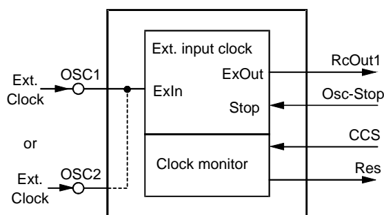
Figure 23. External Input Clock
