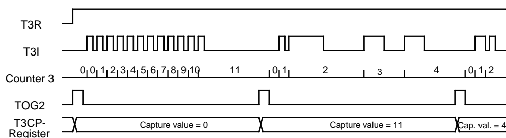
Figure 88. Event Counter with Time Gate
