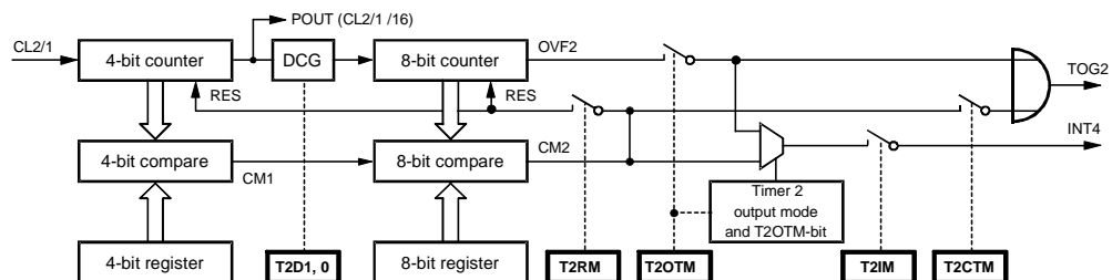
Figure 38. 12-bit Compare Counter
