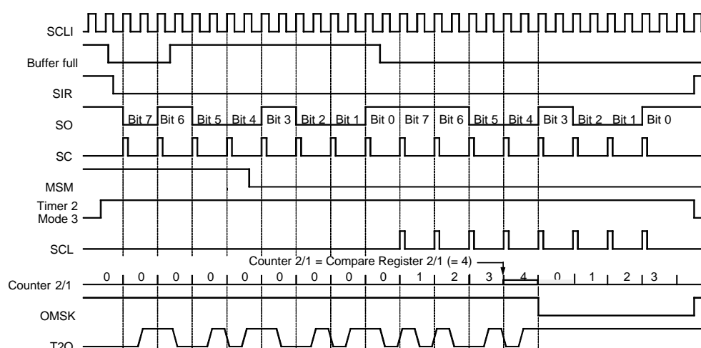
Figure 79. Manchester Modulation 2
