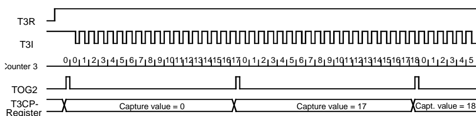
Figure 87. Frequency Measurement
