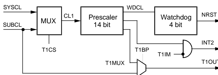
Figure 35. Timer 1 Module
