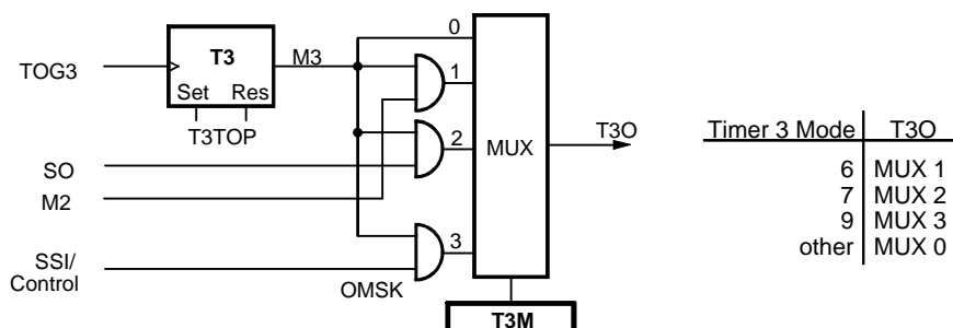
Figure 63. Modulator 3
