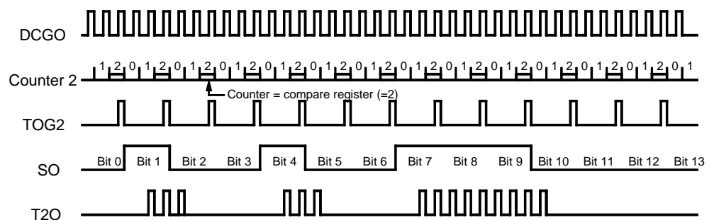
Figure 46. Carrier Frequency Burst Modulation with the SSI Data Output
