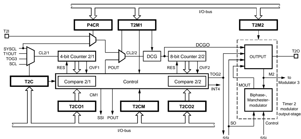
Figure 37. Timer 2
