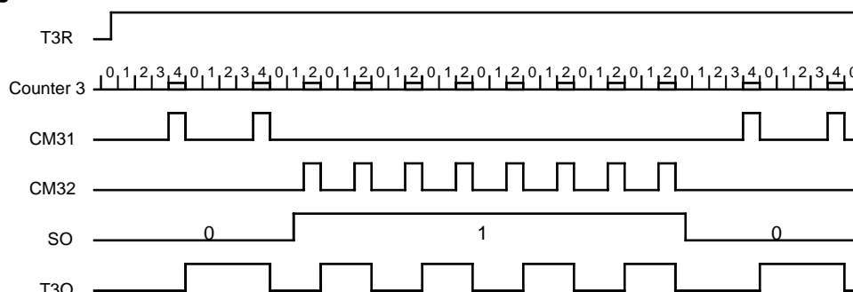
Figure 82. FSK Modulation
