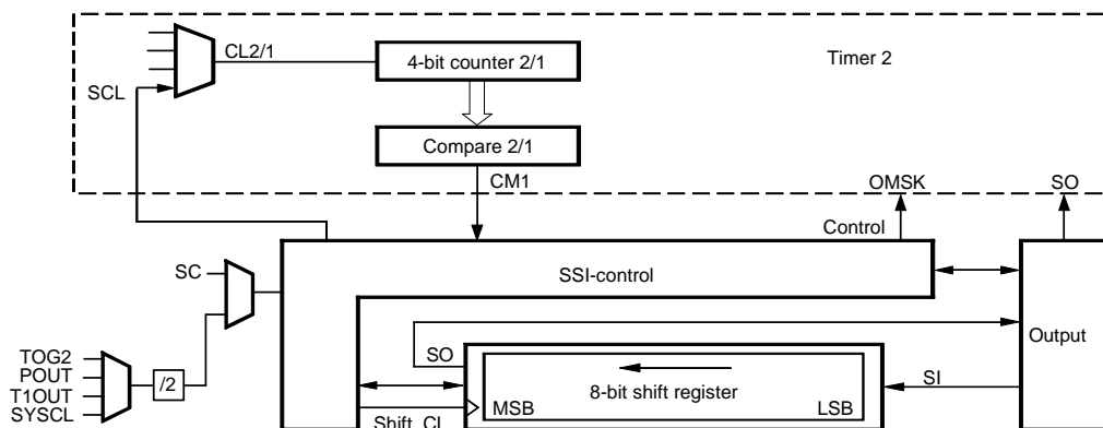
Figure 74. SSI Output Masking Function
