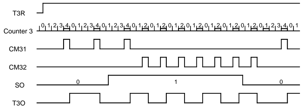
Figure 92. FSK Modulation
