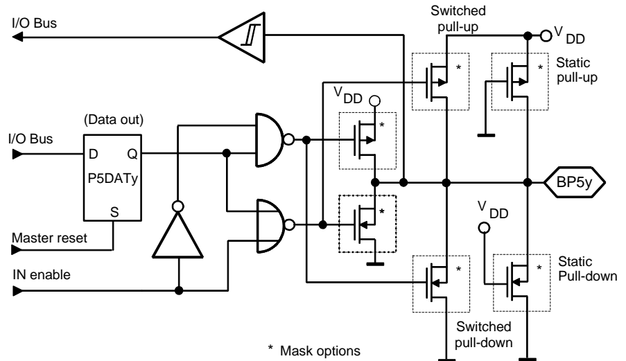
Figure 31. Bi-directional Port 5
