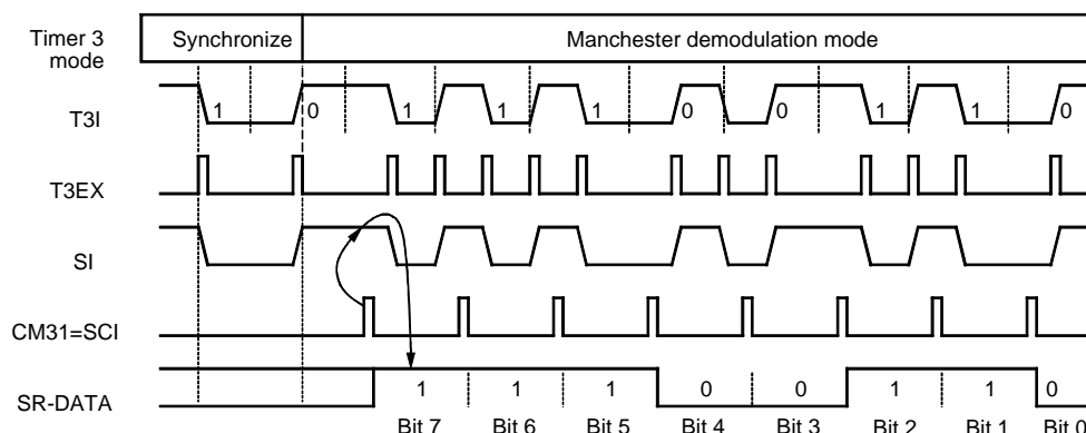
Figure 84. Manchester Demodulation
