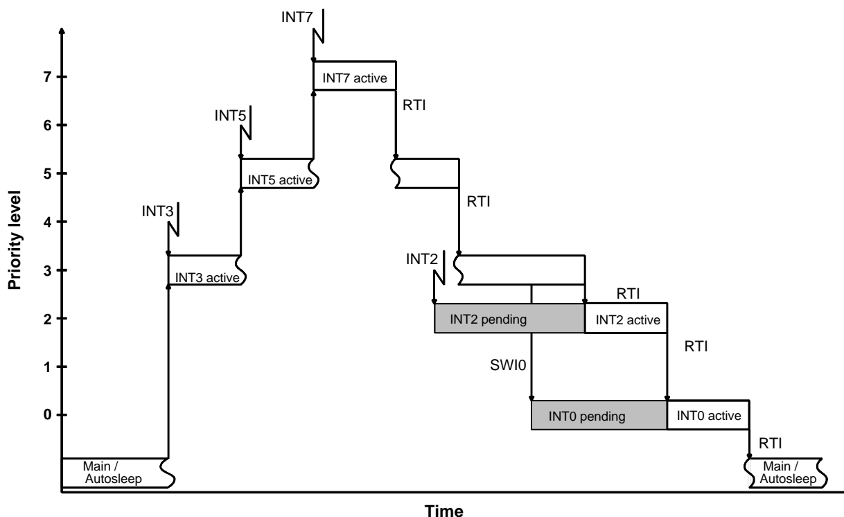
Figure 15. Interrupt Handling
