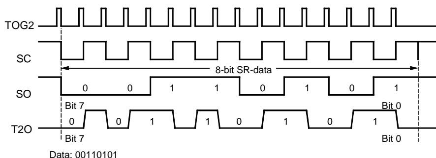
Figure 78. Manchester Modulation 1
