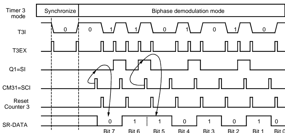
Figure 85. Biphase Demodulation
