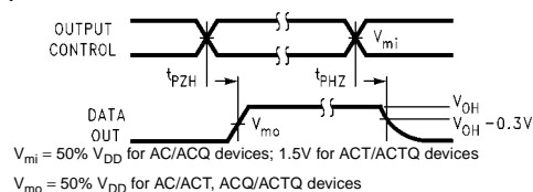
FIGURE 8. 3-STATE Output High Enable and Disable Times for AC/ACT, ACQ/ACTQ
