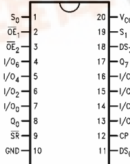
Pin Assignment for DIP
