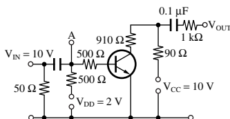
t_{stg} Test circuit
