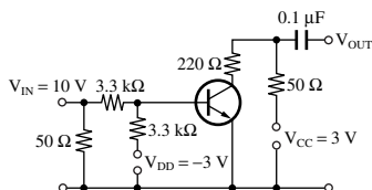
t_{on} , t_{off} Test circuit
