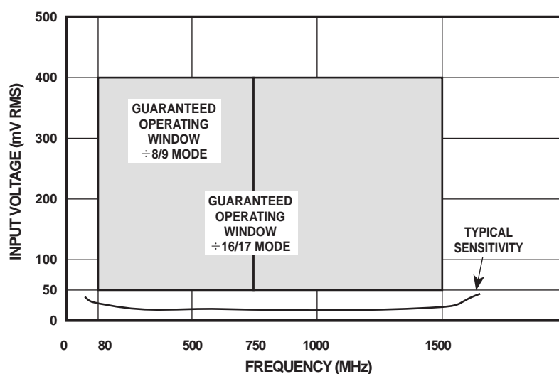
Fig. 3 Typical input characteristics and input drive requirements
