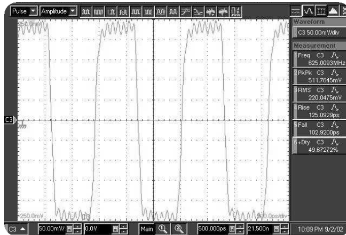
Figure 12 - Output waveform-single-ended VCC=5V, Vin=2dBm, Fin=10GHz
