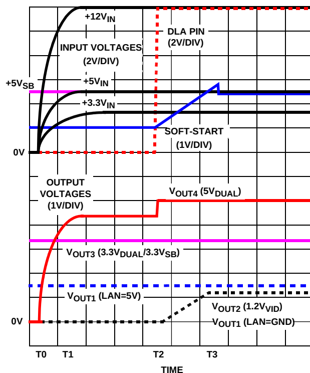
FIGURE 9. SOFT-START INTERVAL IN ACTIVE STATE
