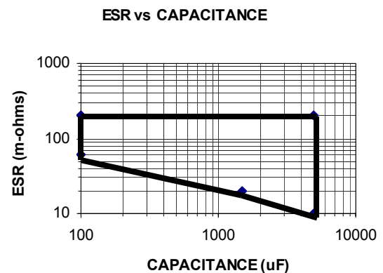
FIGURE 11. V OUT1 OUTPUT CAPACITOR SELECTION
