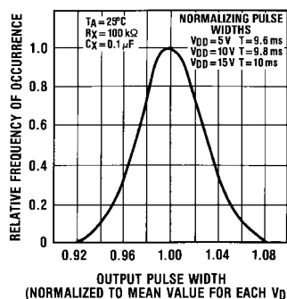
FIGURE 6. Typical Normalized Distribution of Units for Output Pulse Width
