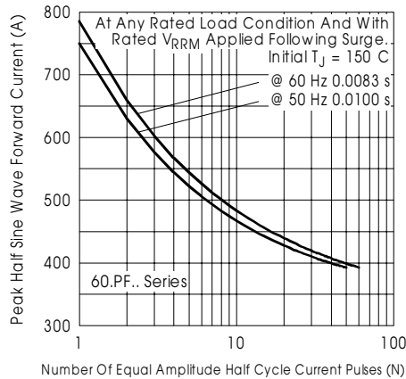
Fig.5-MaximumNon-RepetitiveSurgeCurrent
