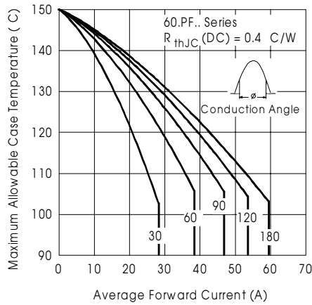
Fig.1-CurrentRatingCharacteristics
