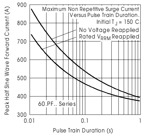
Fig.6-MaximumNon-RepetitiveSurgeCurrent
