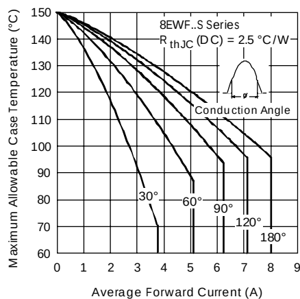
Fig.1-Current Rating Characteristics
