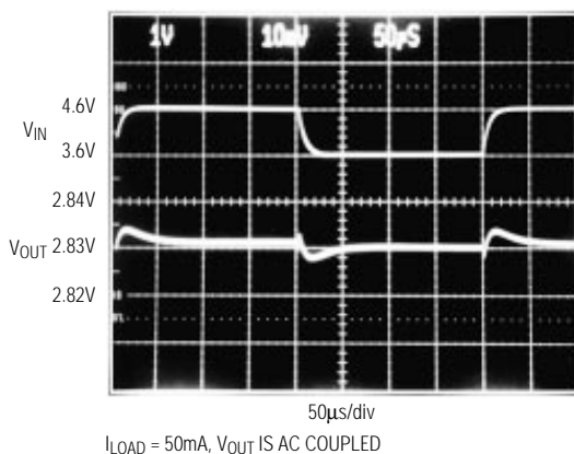
LINE-TRANSIENT RESPONSE
