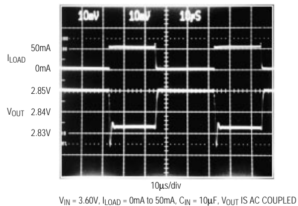
LOAD-TRANSIENT RESPONSE
