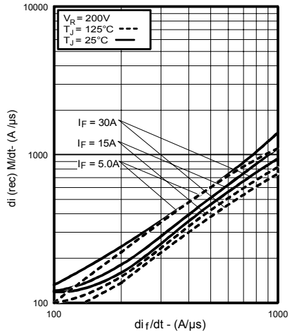
Fig. 8 - Typical di_{(rec)}M/dt vs. di_f/dt , (per Leg)
