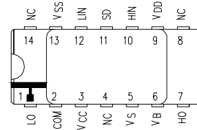
LEAD ASSIGNMENTS
