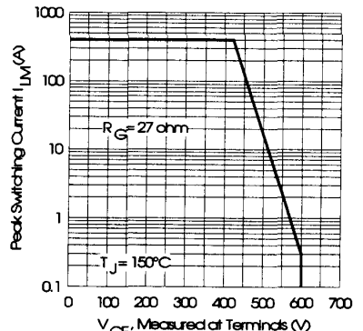
Fig. 12 - Typical Peak Switching Current vs. Measured at Terminals Voltage
