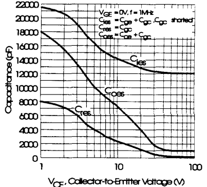
Fig. 8 - Typical Capacitance vs. Collector-to-Emitter Voltage
