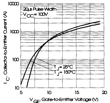
Fig. 4 - Typical Transfer Characteristics
