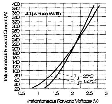
Fig. 6 - Forward Voltage Drop Characteristics
