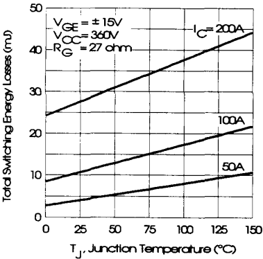
Fig. 9 - Typical Switching Losses vs. Junction Temperature
