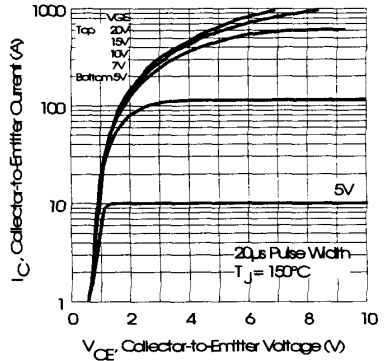
Fig. 2 - Typical Output Characteristics, T_J = 150^\circ\text{C}
