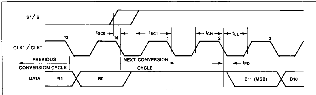
Figure 5. MAX171 Timing Diagram
