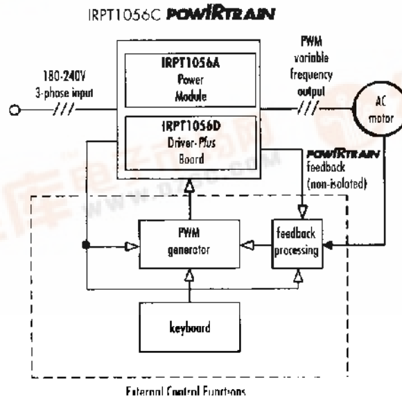
Figure 2. The power module and POWIRTRAIN within a
