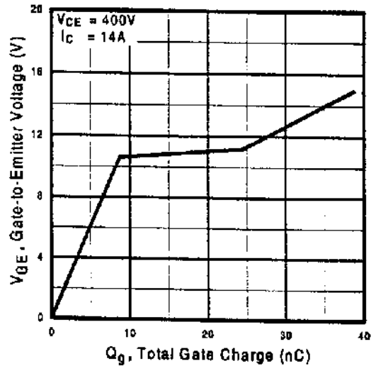
Figure 5b. Typical Gate Charge vs Gate-to-Emitter Voltage
