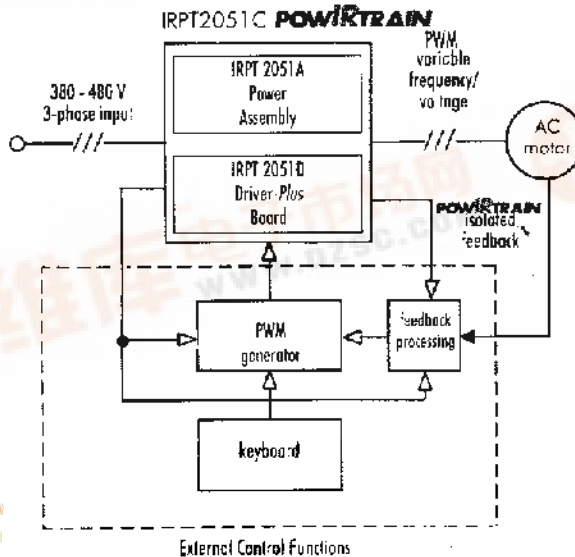
Figure 2. The IRPT2051C POWERTRAIN within a motor
