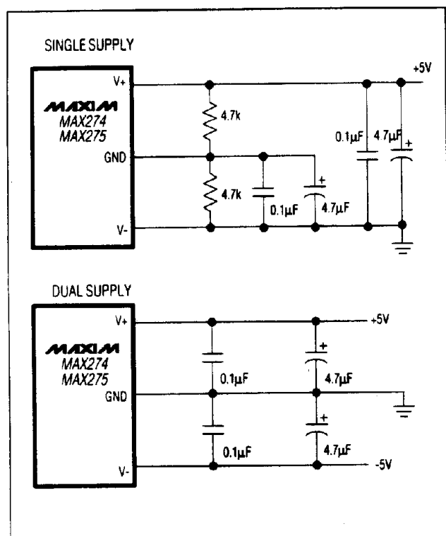
Figure 9. Power-Supply Configurations
