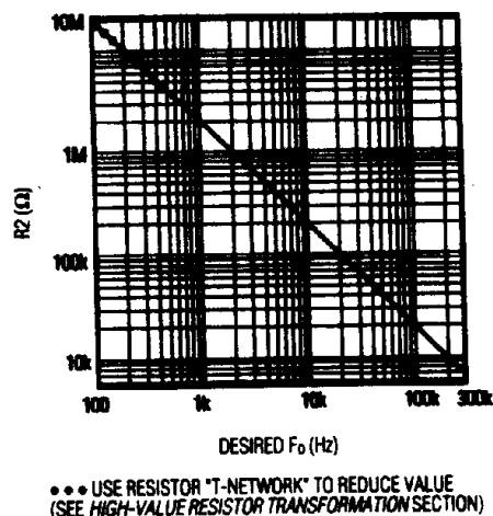
RESISTOR R2 vs. DESIRED CENTER FREQUENCY
