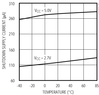
MAX961/MAX963/MAX964/MAX997 SHUTDOWN SUPPLY CURRENT PER COMPARETOR vs. TEMPERATURE
