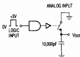
Figure 2. Charge Injection
