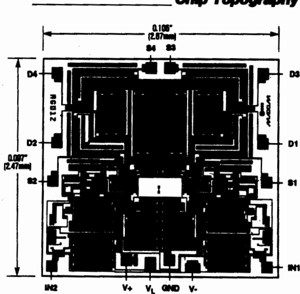
Chip Topography
