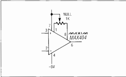
Figure 7. Offset Null Circuit
