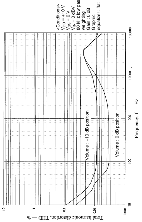
THD—Frequency Characteristics (2)
