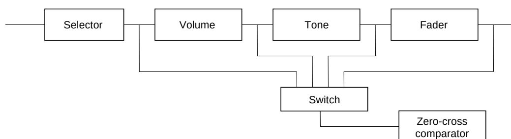
LC75412E, 75412W Zero-Cross Detection Circuit
