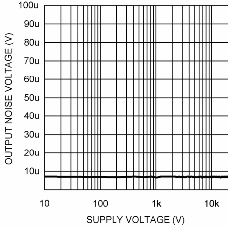
Noise Floor V_{DD} = 1.5V , Single Ended Output 16\Omega , 80kHz Bandwith
