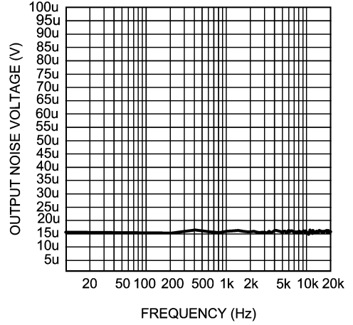
Noise Floor V_{DD} = 1.5V , BTL Output 8\Omega , 80kHz Bandwith
