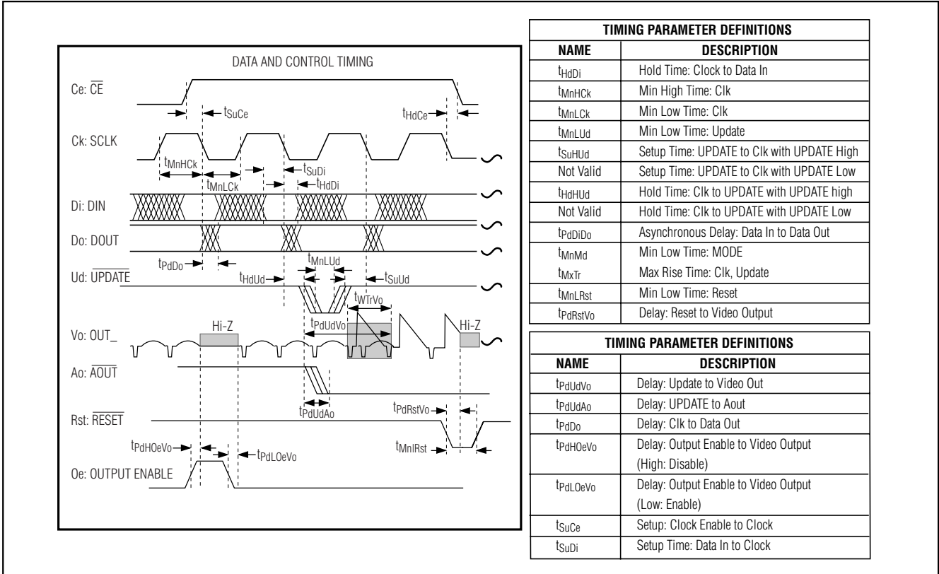
Figure 1. Timing Diagram
