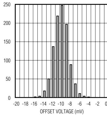
OFFSET VOLTAGE HISTOGRAM
