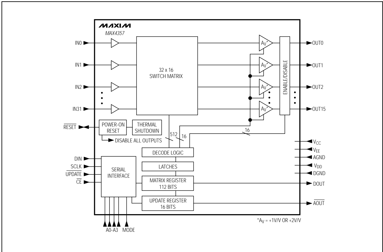
Functional Diagram
