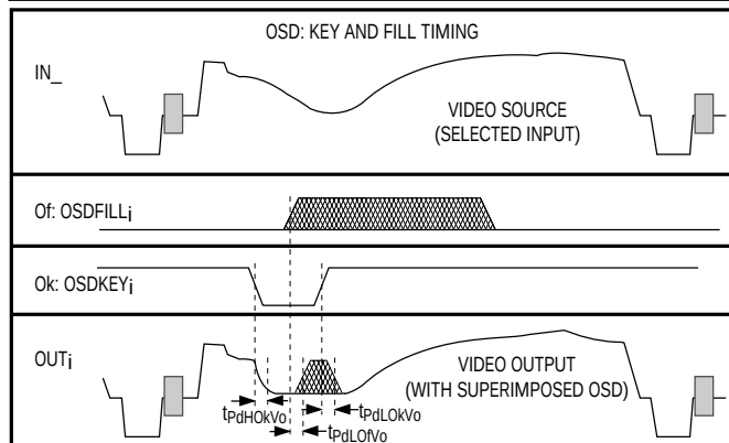
Figure 1. Timing Diagram
