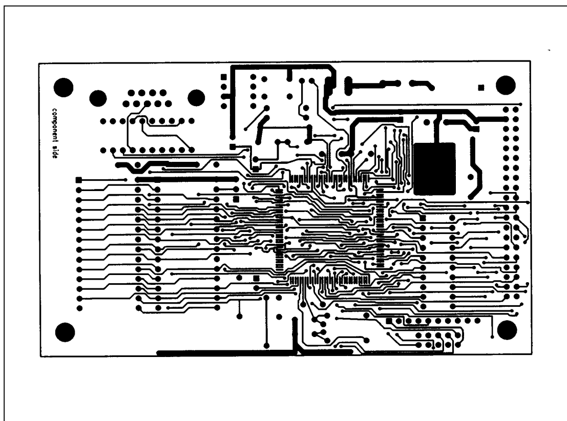
Figure 7. 68HC16 Module PC Board Layout—Component Side
