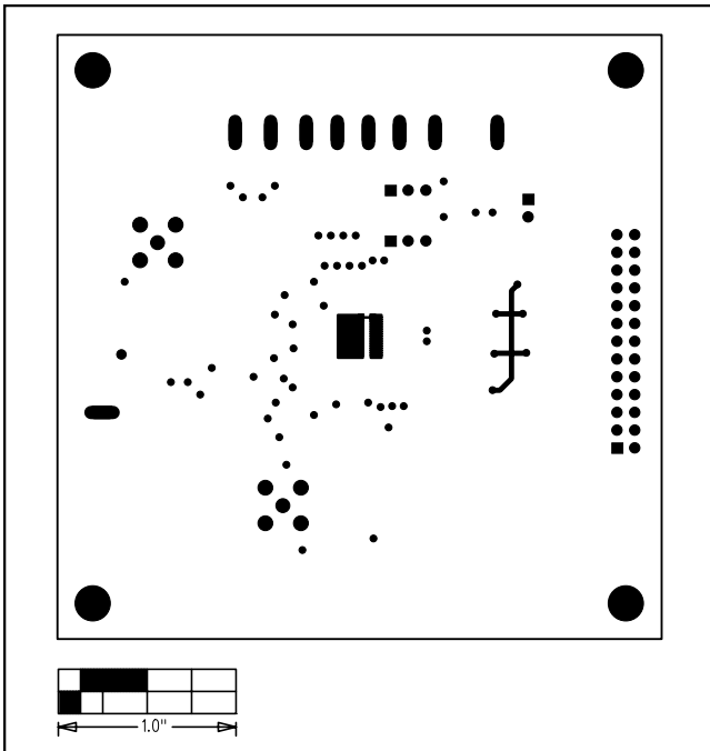
Figure 4. MAX1420 EV Kit PC Board Layout—Solder Side
