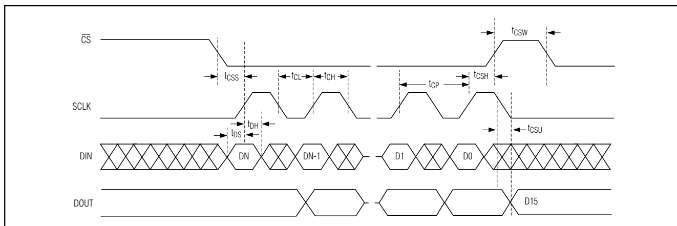
Figure 8. 4-Wire Serial Interface Timing Diagram
