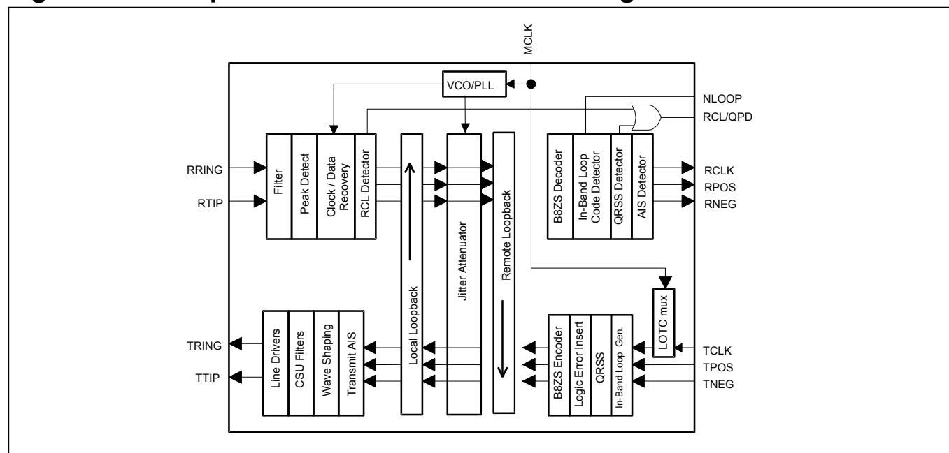
Figure 10-1. Loopbacks in the DS21349 Block Diagram
