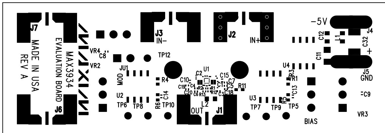
Figure 2. MAX3934 EV Kit Component Placement Guide—Component Side
