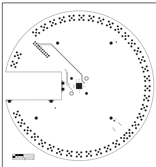
Figure 7. MAX3953 EV Kit PC Board Layout—Solder Side
