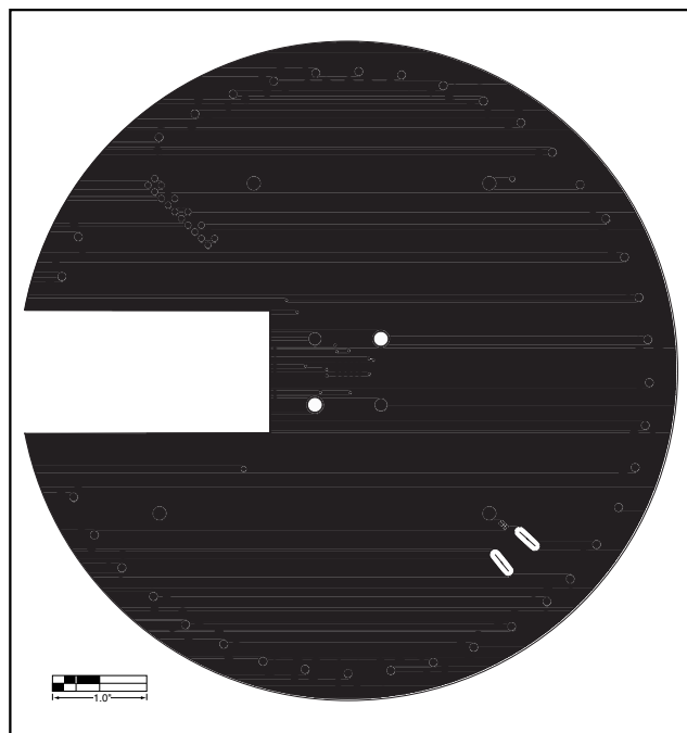
Figure 5. MAX3953 EV Kit PC Board Layout—Ground Plane
