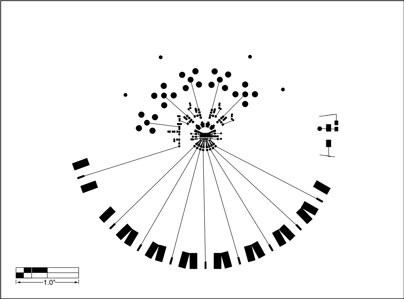
Figure 3. MAX3825 Evaluation Kit PC Board Layout—Component Side
