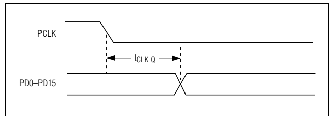
Figure 2. Timing Parameters
