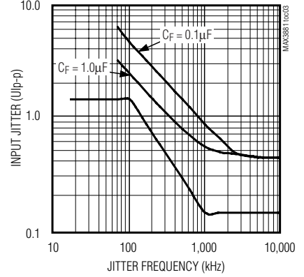
JITTER TOLERANCE
