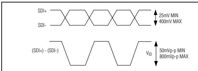
Figure 1. Input Amplitude
