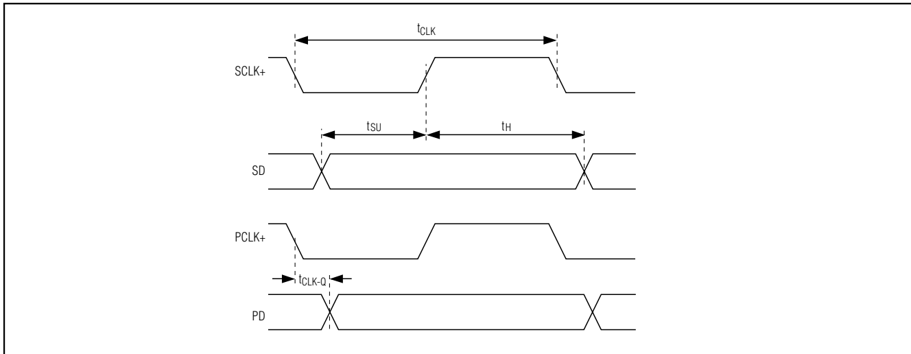
Figure 3. Timing Parameters
