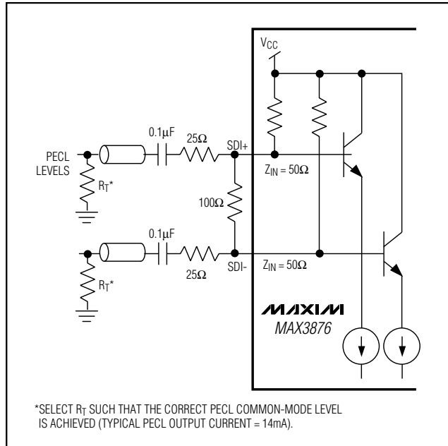
Figure 7. PECL-to-CML Interface
