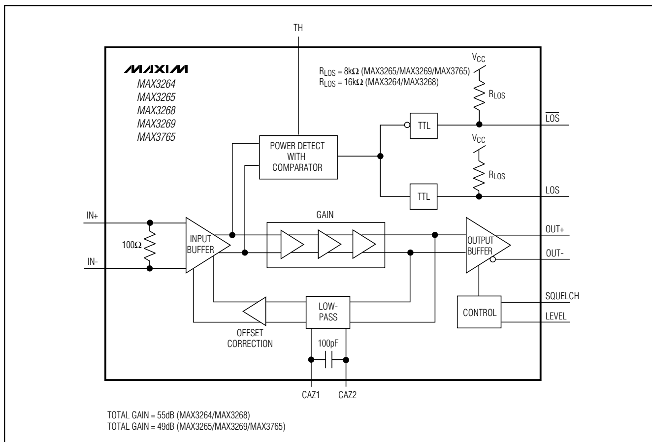
Figure 3. Functional Diagram
