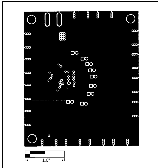
Figure 7. MAX3680 EV Kit PC Board Layout—Power Plane*
