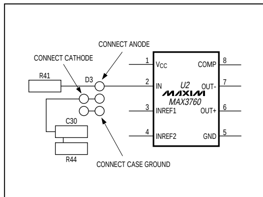
Figure 1. Photodiode Connection
