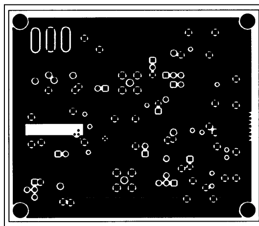
Figure 4. MAX3762 EV Kit PC Board Layout—Ground Plane
