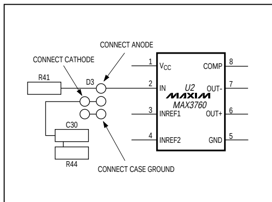
Figure 1. Photodiode Connection
