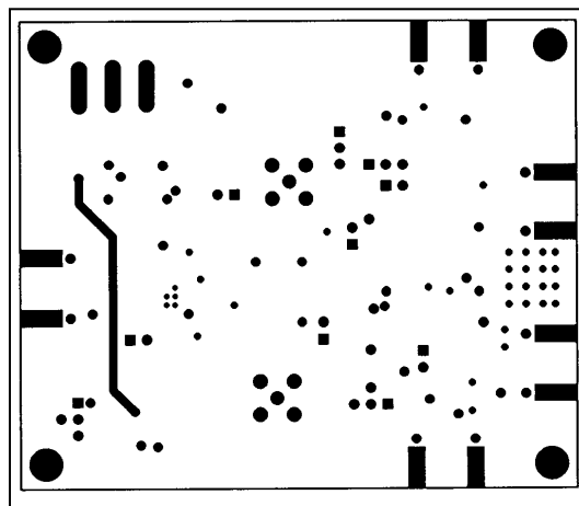
Figure 6. MAX3762 EV Kit PC Board Layout—Solder Side
