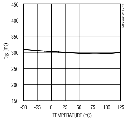
RESTART DELAY vs. TEMPERATURE
