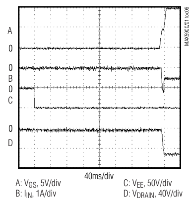
STARTUP WAVEFORMS R_L = 90\Omega , C_L = 100\mu F
