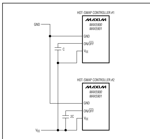
Figure 3. Power-Supply Sequencing
