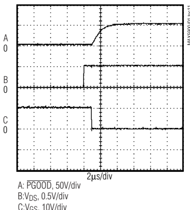
CIRCUIT BREAKER EVENT ( C_{GATE} = 1000pF , V_{OVERDRIVE} = 200mV )
