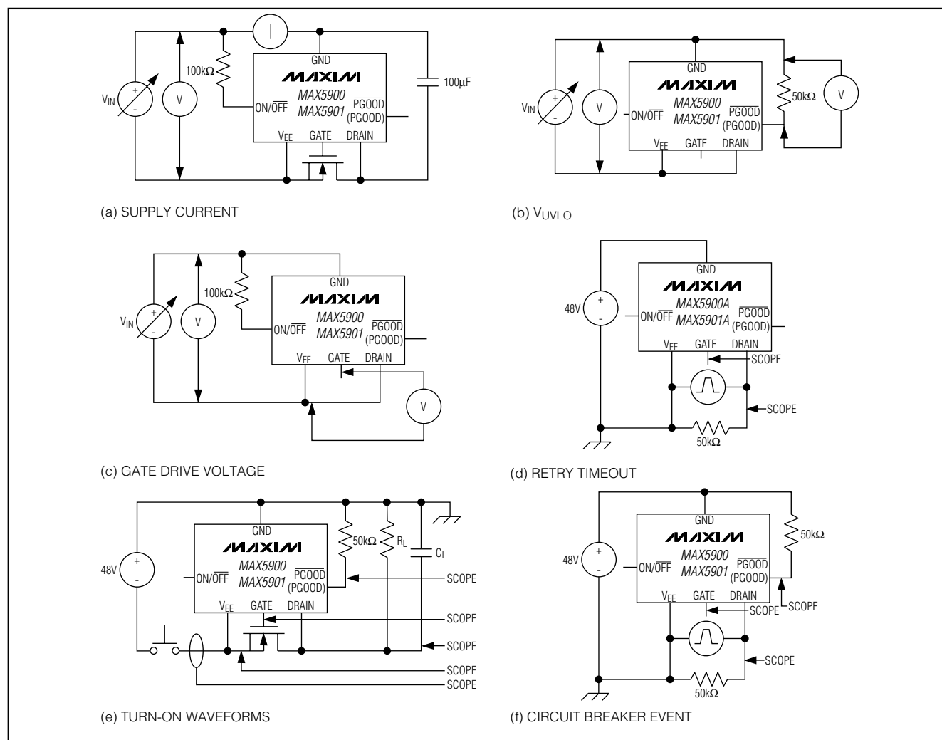
Figure 6. Test Circuits
