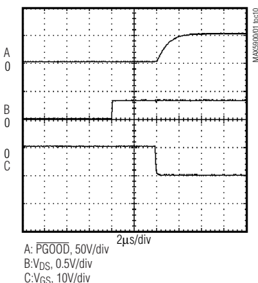
CIRCUIT BREAKER EVENT ( C_{GATE} = 1000pF , V_{OVERDRIVE} = 20mV )
