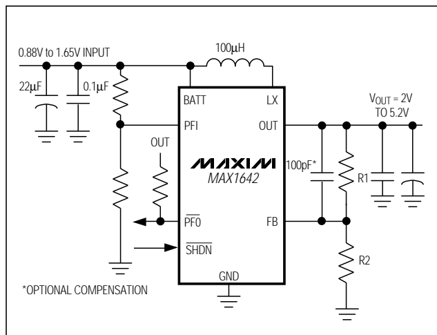
Figure 4. Adjustable-Output Circuit
